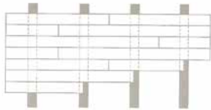
(Fig 4) End matched joints should be staggered and are not to occur in adjacent boards within the same span.
