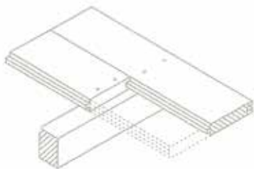
(Fig 6) Top Nail.
