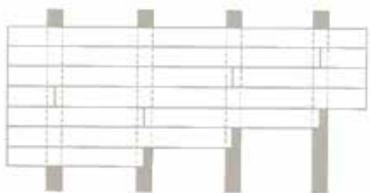
(Fig 5) Butt joints over joists should be staggered and are not to occur in adjacent boards on the same joist.
