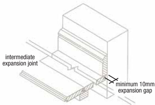
(Fig 3) Edge gap & intermediate expansion joint.
