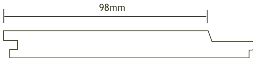
110 X 12 SHIPLAP LINING
