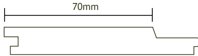
85 X 12 SHIPLAP LINING
