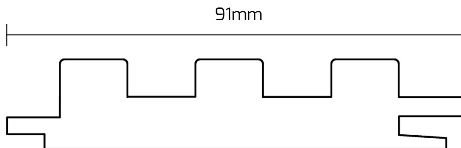
81 x 19 CASTELLATION 3 BATTEN MOULD
