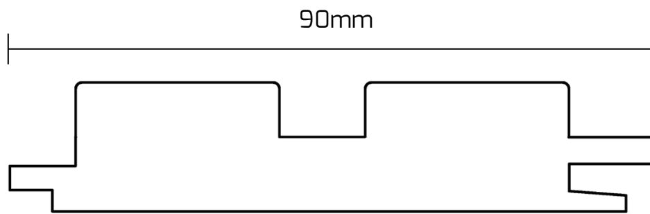
81 X 19 CASTELLATION 2 BATTEN MOULD
