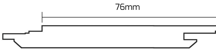
76 x 12 SHIPLAP/VJ LINING
