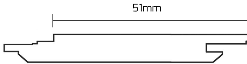
51 x 12 SHIPLAP/VJ LINING
