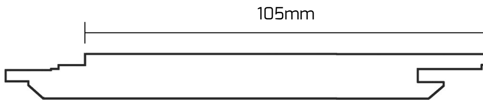
105 x 12 SHIPLAP/VJ LINING
