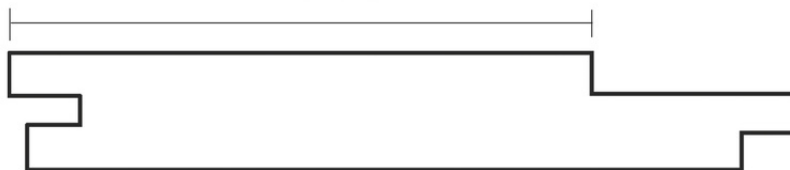
133 x 12 SHIPLAP LINING
