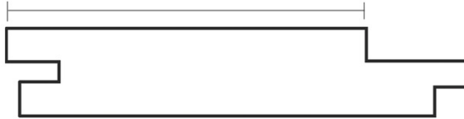
85 X 12 SHIPLAP LINING
