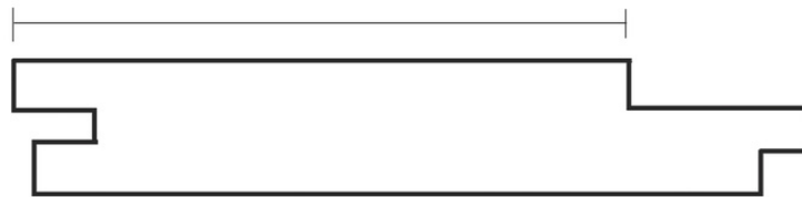
110 x 12 SHIPLAP LINING
